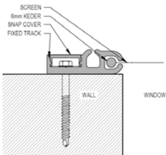
① SECTION - FACE MOUNT SCALE: 12" = 1'-0"
