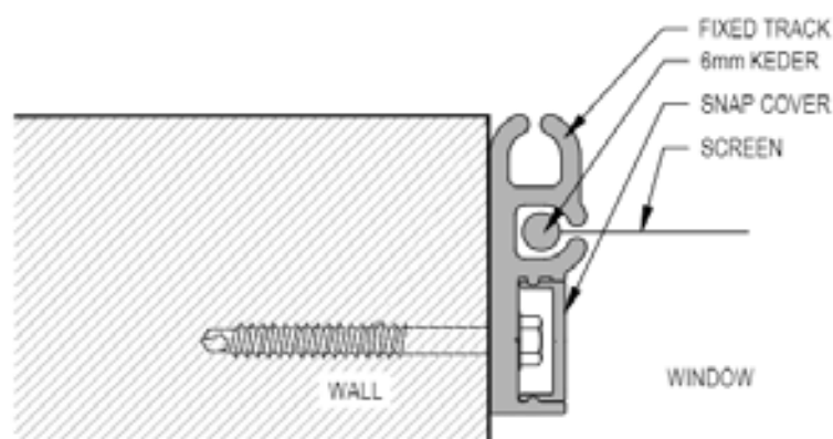
② SECTION - INSIDE MOUNT SCALE: 12" = 1'-0"
